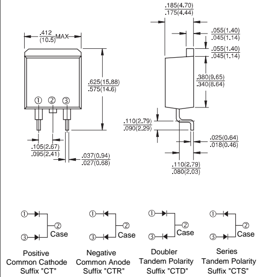
D2PAK/TO-263
