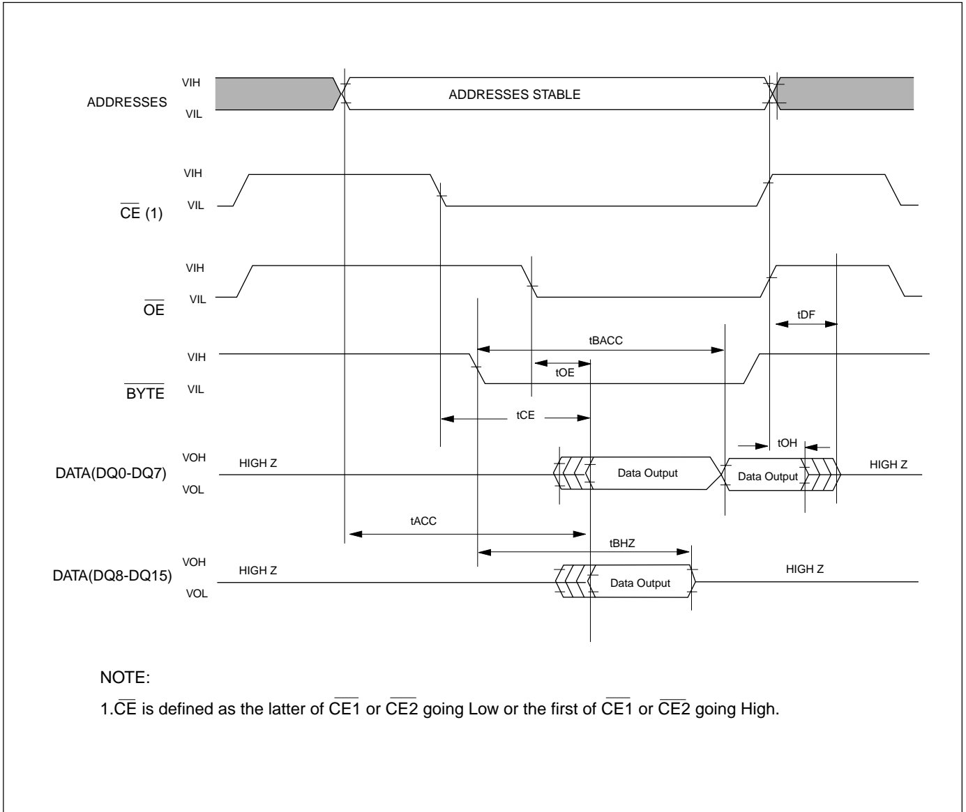
Figure 6. BYTE TIMING WAVEFORMS
