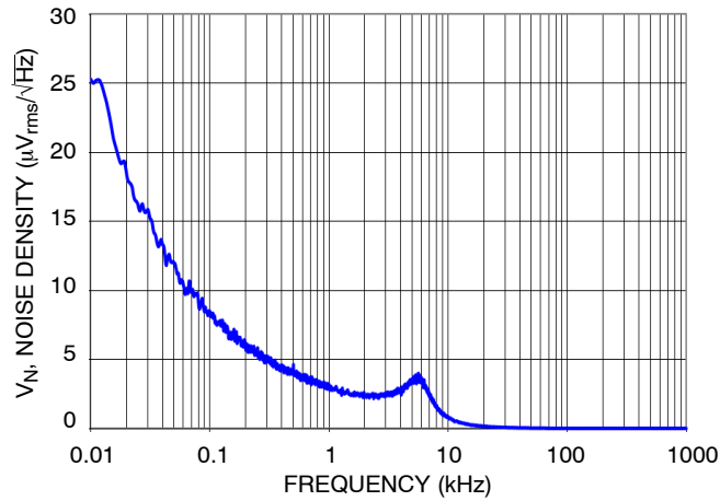
Figure 23. Output Noise Density, V_{OUT} = 12\text{ V}
