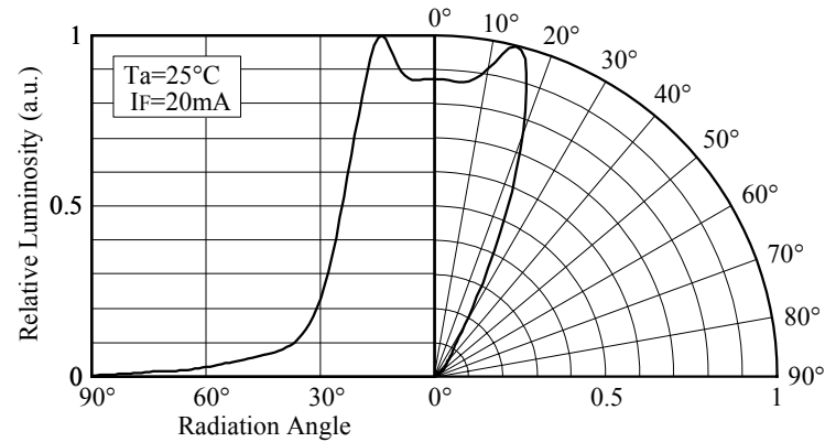
■ Directivity (NSPW510B(S))
