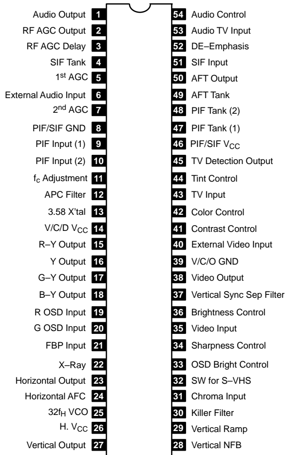
Pin Connection Diagram
