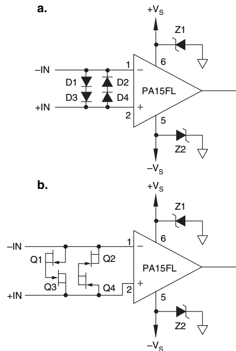
FIGURE 2. OVERVOLTAGE PROTECTION
