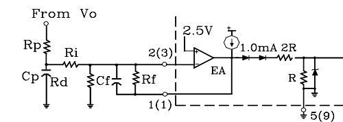
FIGURE 31-ERROR AMPLIFIER COMPENSATION
