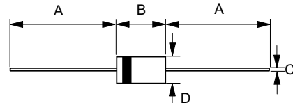
DO-41
