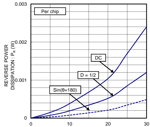
V_R -P R CHARACTERISTICS
