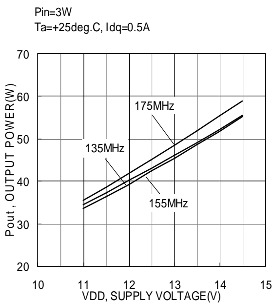
Output Power versus Supply Voltage
