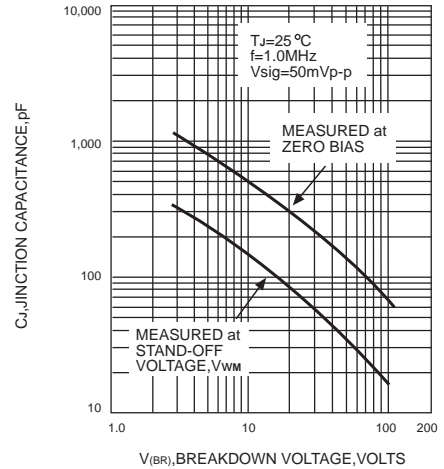
FIG. 4-TYPICAL JUNCTION CAPACITANCE UNIDIRECTIONAL
