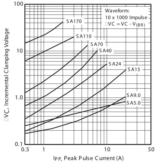
Fig. 8D Incremental Clamping Voltage Curve Unidirectional
