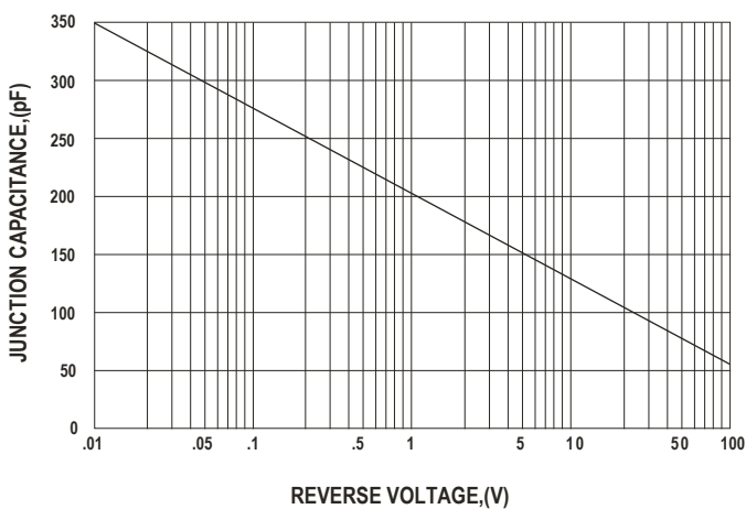
FIG.4-TYPICAL JUNCTION CAPACITANCE
