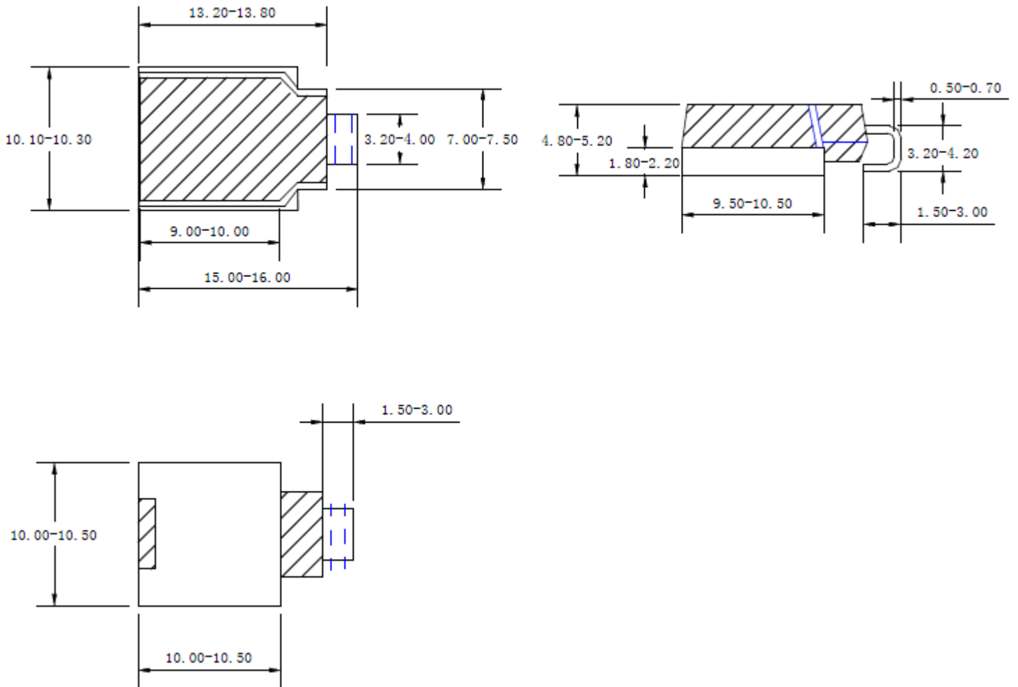
DO-218AB/SMD-BLOCK (mm)
