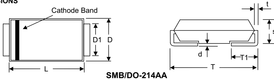
SMB/DO-214AA
