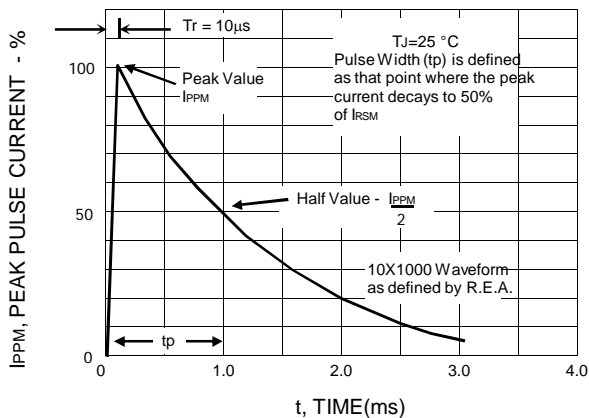
FIG.5 - PULSE WAVEFORM
