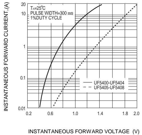
FIG.2-TYPICAL FORWARD CHARACTERISTICS
