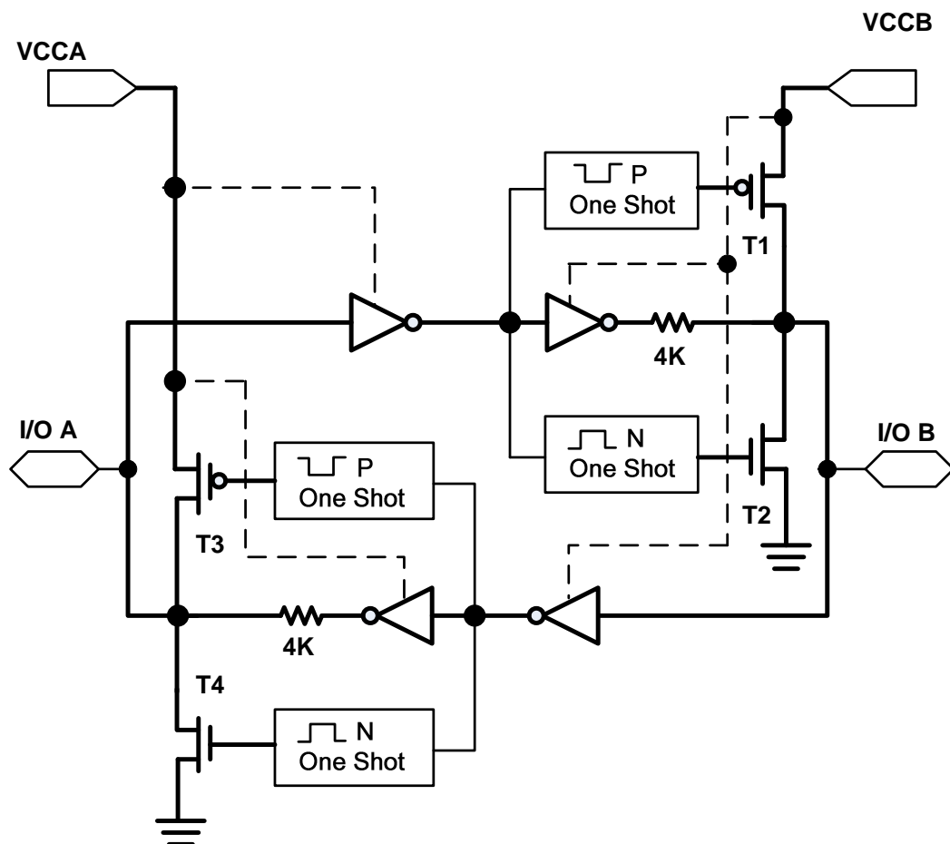
Figure 1 Block Diagram of UM3308 I/O Cell
