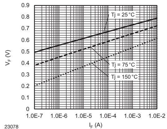
Fig. 6 - Typical Forward Voltage vs. Forward Current
