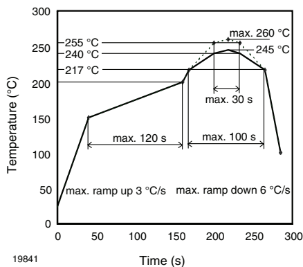
Fig. 11 - Lead (Pb)-free Reflow Solder Profile acc. J-STD-020
