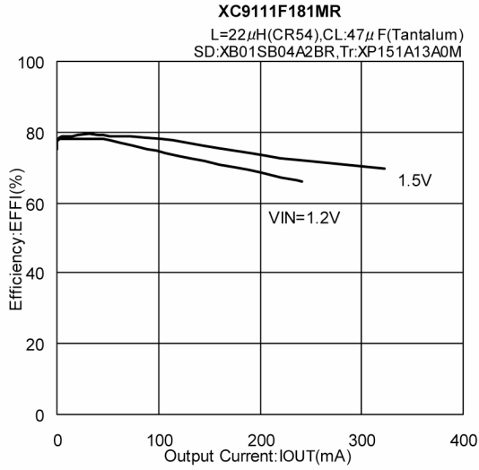
(2) Efficiency vs. Output Current (Continued)
