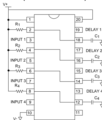
QUAD MONOSTABLE MODE OPERATION (ONE SHOT PULSE)
