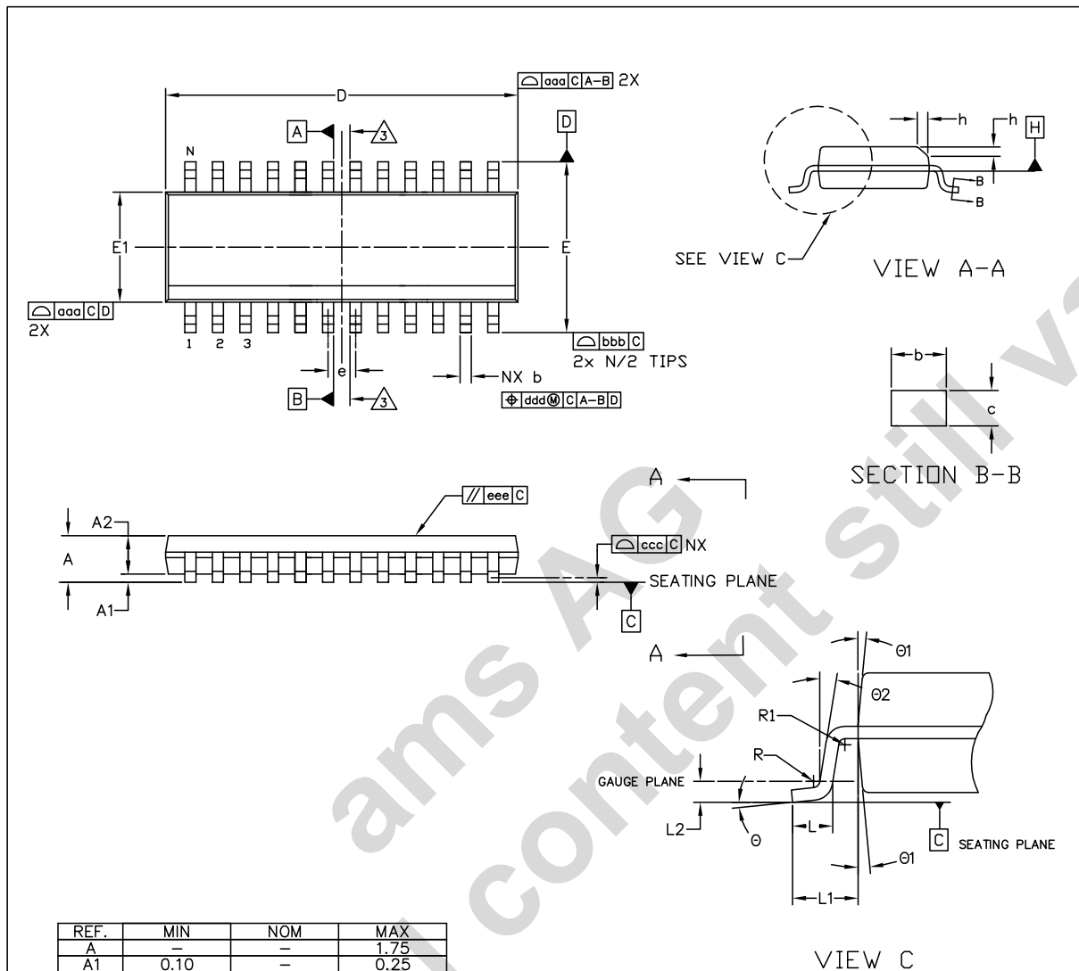
Figure 24. QSOP-24 Package
