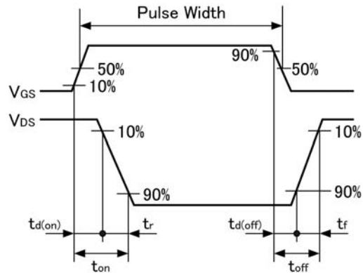
Fig.2 Switching waveforms
