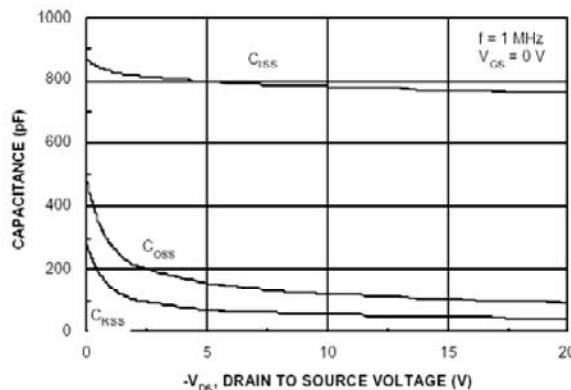
Figure 8. Capacitance Characteristic
