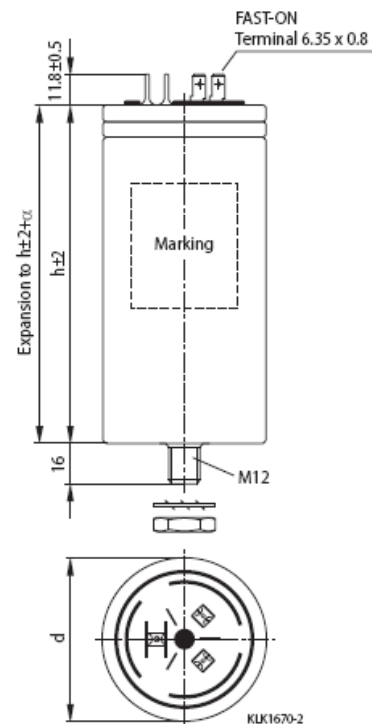
Dimensional drawing
