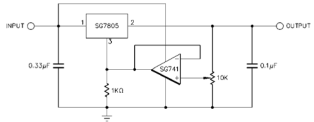
Figure 8 – Adjustable Output Regulator, 7V to 30V
