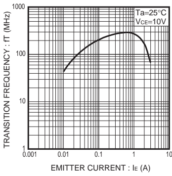
Fig.7 Transition Frequency
