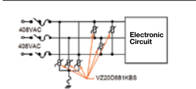
MOV for 3 Phase AC Line Protection
