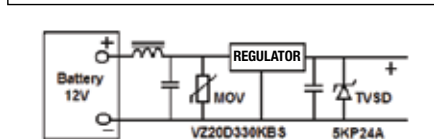
MOV in Automotive Equipment Protection
