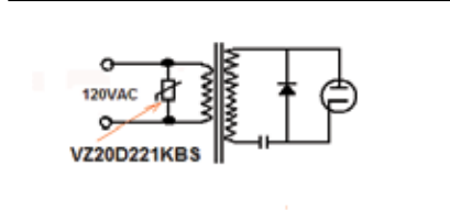
MOV In Microwave Oven
