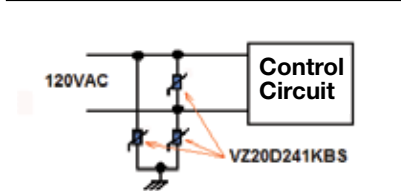
MOV In Control Circuit Protection
