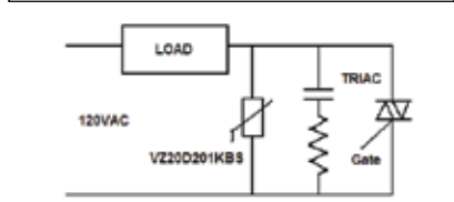
MOV in Triac Protection
