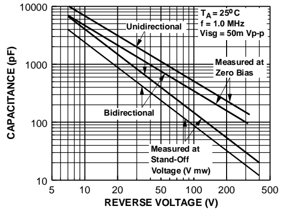
Junction Capacitance
