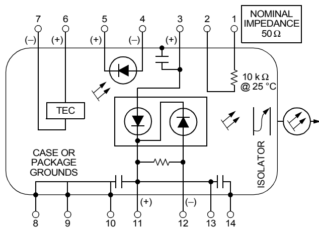
Figure 1. E2500 EM-ILM Schematic
