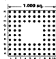
84 PINS Footprint 10003
