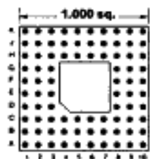
84 PINS Footprint 10002
