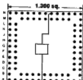
84 PINS Footprint 13056
