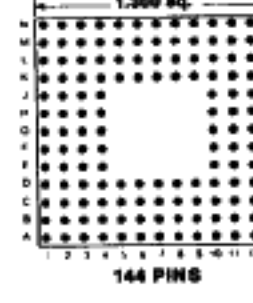
144 PINS Footprint 13003
