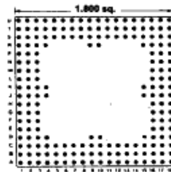
181 PINS Footprint 18010
