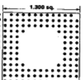
121 PINS Footprint 13058
