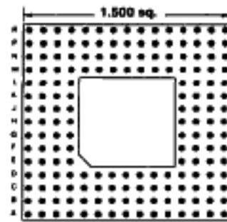
176 PINS Footprint 15013
