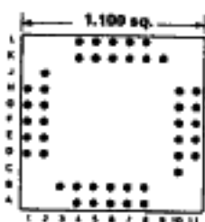
Footprint 11042
