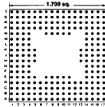
225 PINS Footprint 17007
