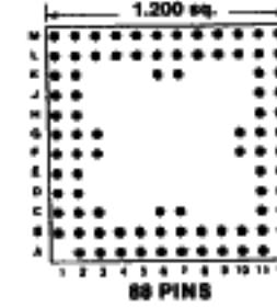
88 PINS Footprint 12009
