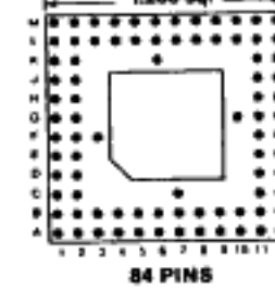
84 PINS Footprint 12010
