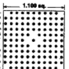
113 PINS Footprint 11004
