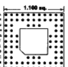
84 PINS Footprint 11009
