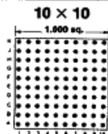
100 PINS Footprint 10001
