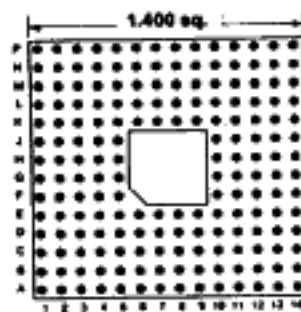
180 PINS Footprint 14002
