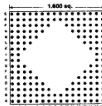
172 PINS Footprint 16002
