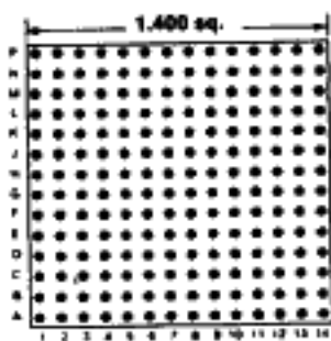
196 PINS Footprint 14001
