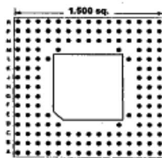
153 PINS Footprint 15016
