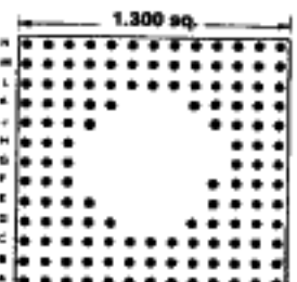
133 PINS Footprint 13052
