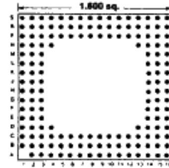
159 PINS Footprint 16009
