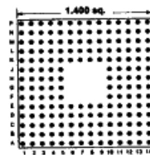
188 PINS Footprint 14003
