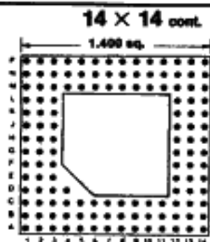
133 PINS Footprint 14013
