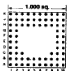
72 PINS Footprint 10004
