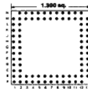
Footprint 13031
