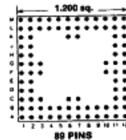
89 PINS Footprint 12007
