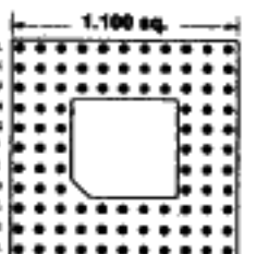
98 PINS Footprint 11005
