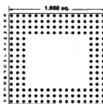
166 PINS Footprint 16004
