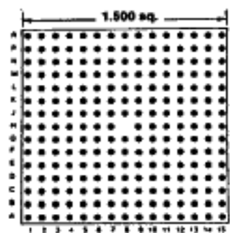
224 PINS Footprint 15038
