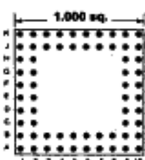
84 PINS Footprint 10010
