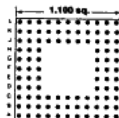
96 PINS Footprint 11006
