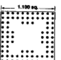
84 PINS Footprint 11010
