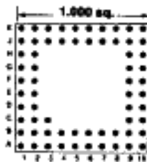
85 PINS Footprint 10008
