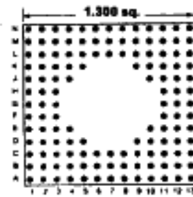
Footprint 13038
