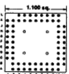
Footprint 11038
