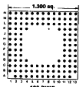
Footprint 13011
