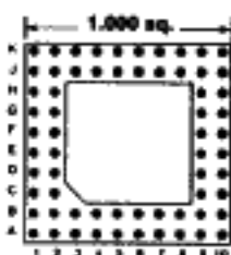
84 PINS Footprint 10009
