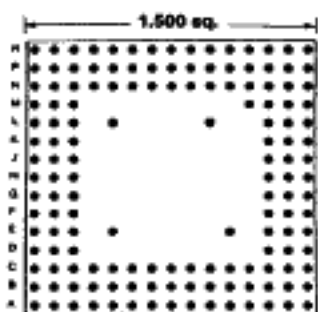
149 PINS Footprint 15020
