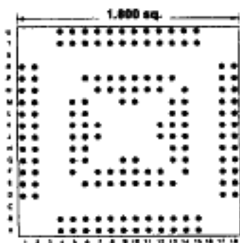
159 PINS Footprint 18008
