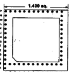
49 PINS Footprint 14019
