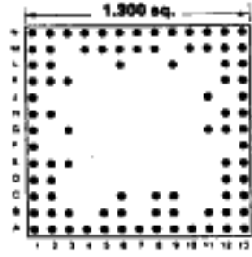
Footprint 13041
