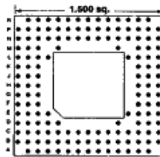
149 PINS Footprint 15018
