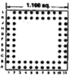
Footprint 11033
