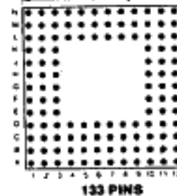
133 PINS Footprint 13005
