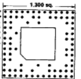
88 PINS Footprint 13049
