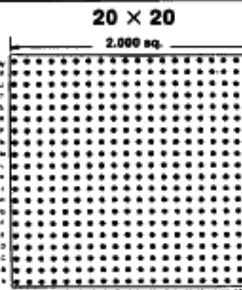
408 PINS Footprint 20001
