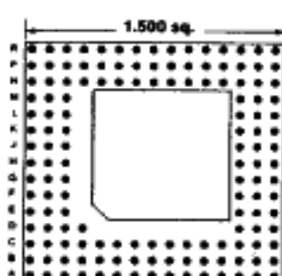
145 PINS Footprint 15023
