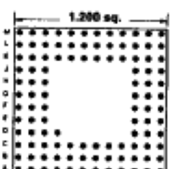
Footprint 12003
