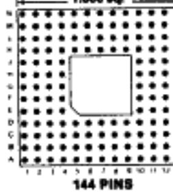
144 PINS Footprint 13002
