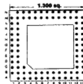
Footprint 13032
