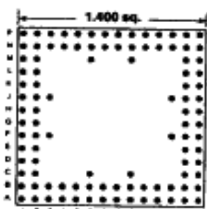
104 PINS Footprint 14018
