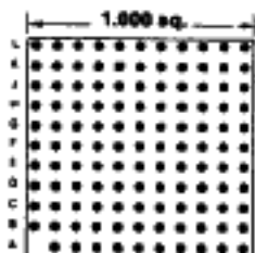
120 PINS Footprint 11002
