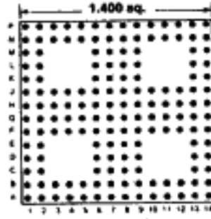
160 PINS Footprint 14009
