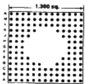
133 PINS Footprint 13046
