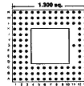
Footprint 13040
