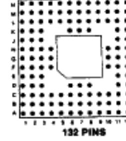
132 PINS Footprint 13006
