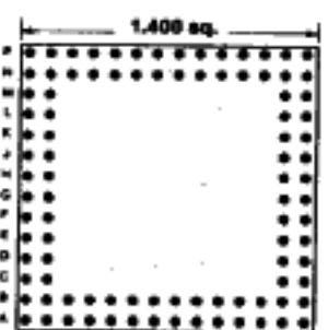
96 PINS Footprint 14024
