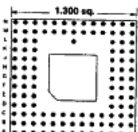
114 PINS Footprint 13051
