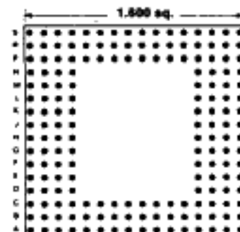
176 PINS Footprint 16007
