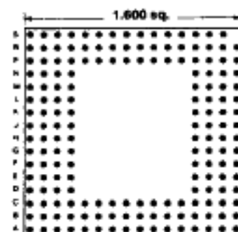
175 PINS Footprint 16008
