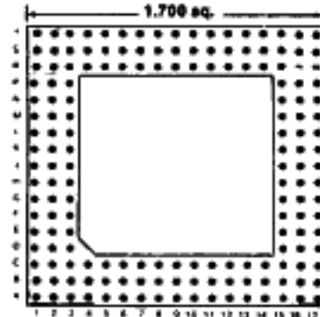
168 PINS Footprint 17009
