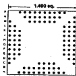
94 PINS Footprint 14022
