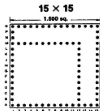
77 PINS Footprint 15037
