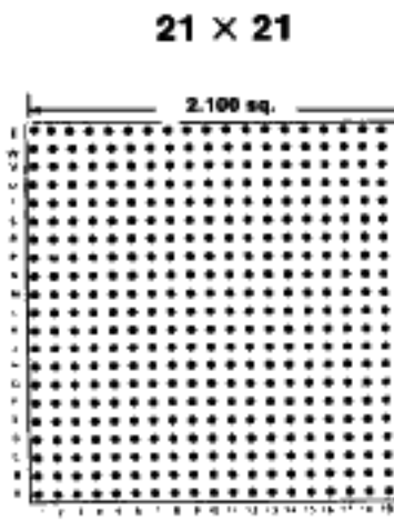
441 PINS Footprint 21001
