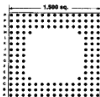
148 PINS Footprint 15022
