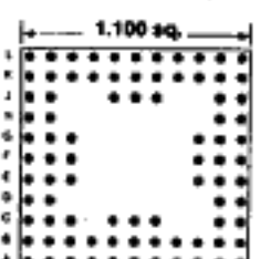
85 PINS Footprint 11008
