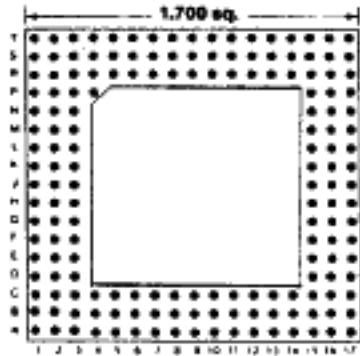
169 PINS Footprint 17010
