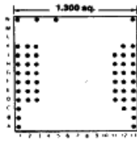
Footprint 13037
