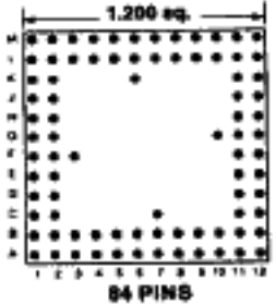
84 PINS Footprint 12011
