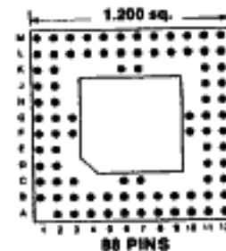
88 PINS Footprint 12008
