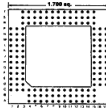
144 PINS Footprint 17005
