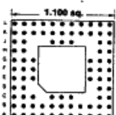
85 PINS Footprint 11007
