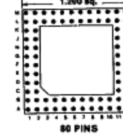
80 PINS Footprint 12014
