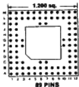
89 PINS Footprint 12006
