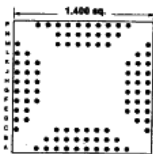
94 PINS Footprint 14023
