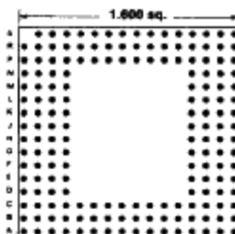
175 PINS Footprint 16003
