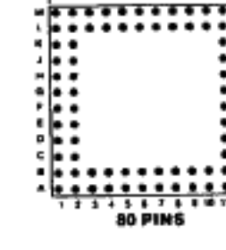
80 PINS Footprint 12015
