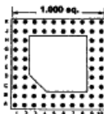
65 PINS Footprint 10007
