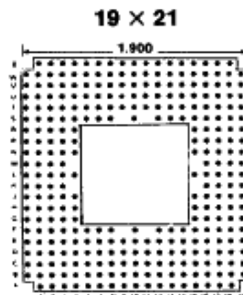
302 PINS Footprint PGA-302
