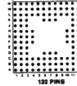
132 PINS Footprint 13007
