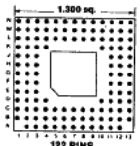
Footprint 13010
