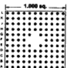
116 PINS Footprint 11003
