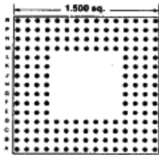
176 PINS Footprint 15014
