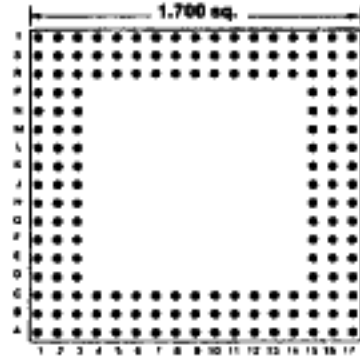
169 PINS Footprint 17011
