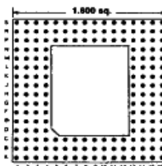
176 PINS Footprint 16006
