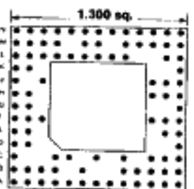
95 PINS Footprint 13047
