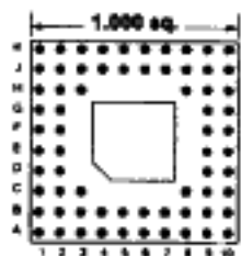
88 PINS Footprint 10005
