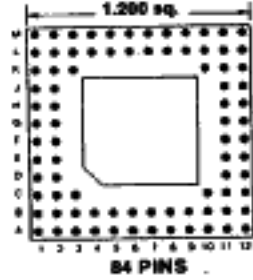
84 PINS Footprint 12012
