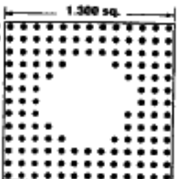
133 PINS Footprint 13054
