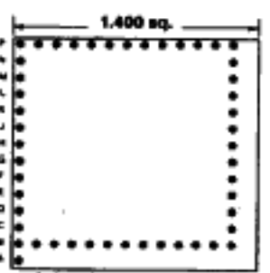
49 PINS Footprint 14020
