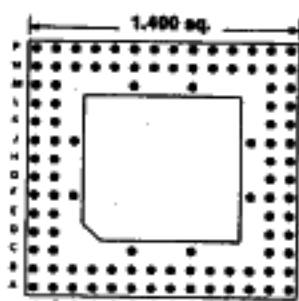
104 PINS Footprint 14017
