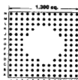
133 PINS Footprint 13055
