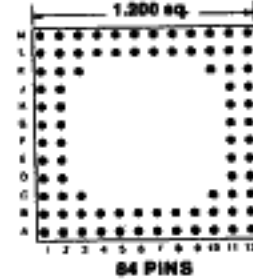
84 PINS Footprint 12013
