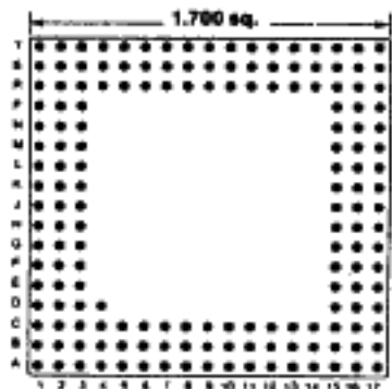
169 PINS Footprint 17012
