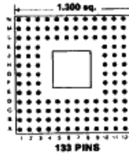
133 PINS Footprint 13004
