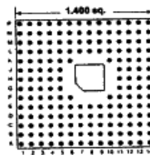
175 PINS Footprint 14004
