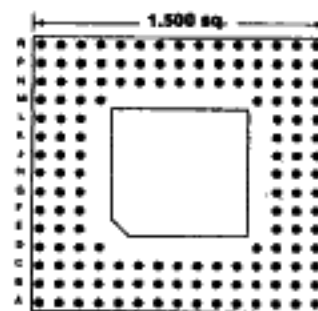
148 PINS Footprint 15021
