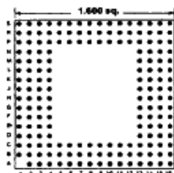
175 PINS Footprint 16010
