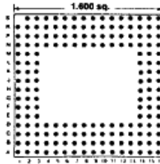
175 PINS Footprint 16005
