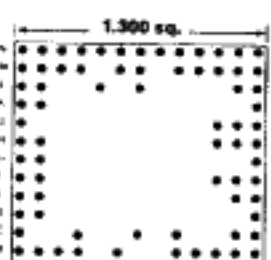
88 PINS Footprint 13057
