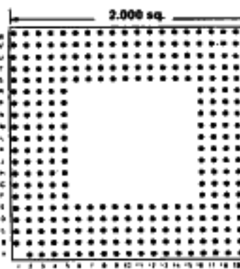
299 PINS Footprint 20002
