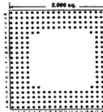
262 PINS Footprint 20003
