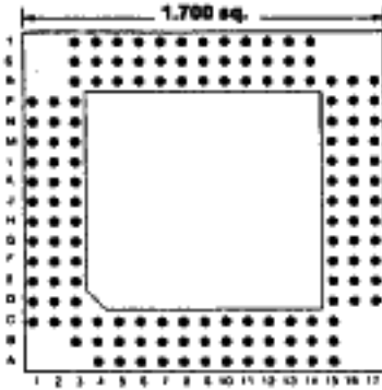
145 PINS Footprint 17003
