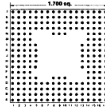
225 PINS Footprint 17008
