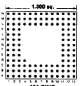
Footprint 13013
