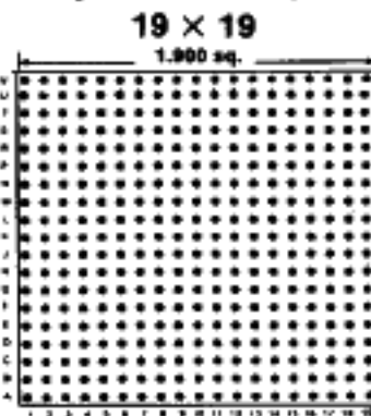
361 PINS Footprint 19001
