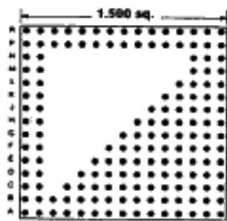
160 PINS Footprint 15015
