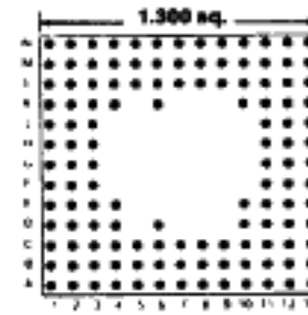
Footprint 13039
