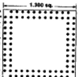
84 PINS Footprint 13053
