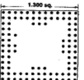
160 PINS Footprint 13059
