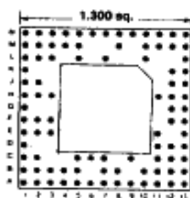
93 PINS Footprint 13045
