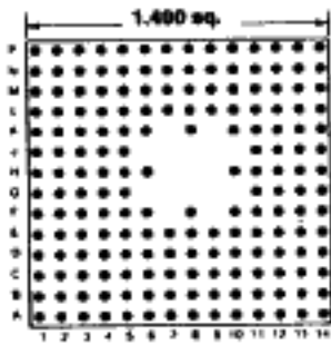
179 PINS Footprint 14005
