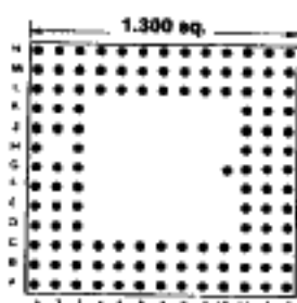
113 PINS Footprint 13050
