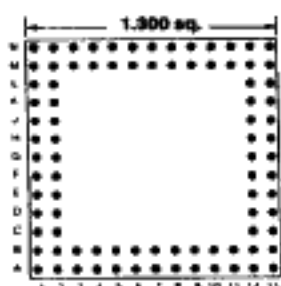
Footprint 13029
