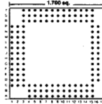
144 PINS Footprint 17006
