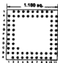
Footprint 11031
