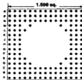
153 PINS Footprint 15017
