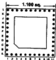
Footprint 11043
