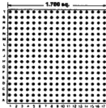
289 PINS Footprint 17001
