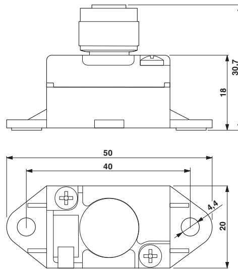
Dimensioned drawing
