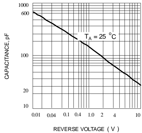
Fig. 4-TYPICAL JUNCTION CAPACITANCE
