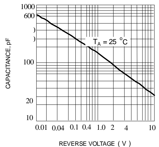
Fig. 4-TYPICAL JUNCTION CAPACITANCE
