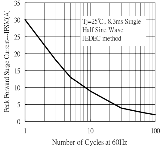
Maximum Non-Repetitive Forward Surge Current
