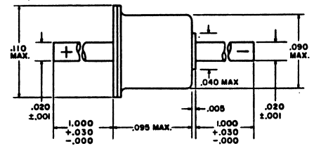
ALL DIMEN. IN INCHES AND ARE REFERENCE UNLESS TOLERANCED.
