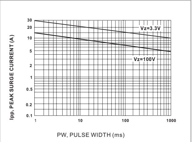
Fig.3 Peak Surge Current versus Pulse Width
