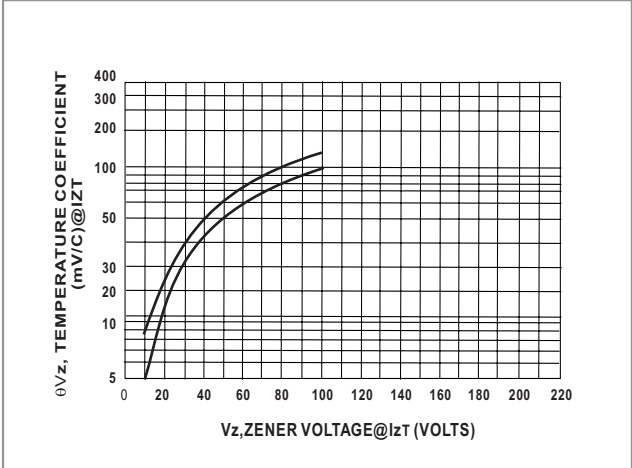
Fig.2 Temperature Coefficient-Range for Units 10 to 100 Volts
