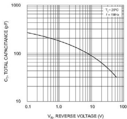
Fig. 5 Typical Total Capacitance
