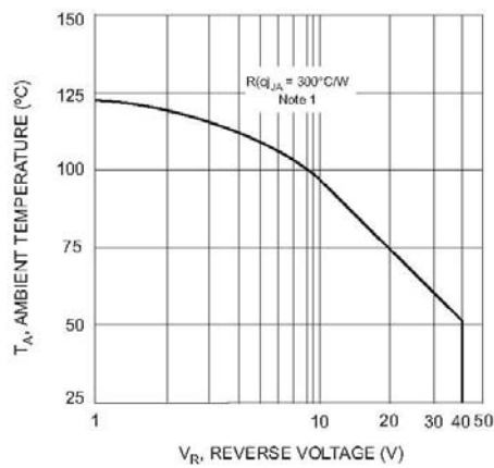
Fig. 3 Typical Safe Operating Area
