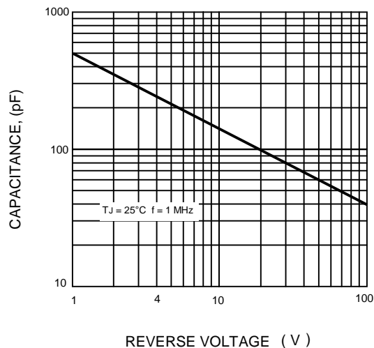
FIG.4-TYPICAL JUNCTION CAPACITANCE
