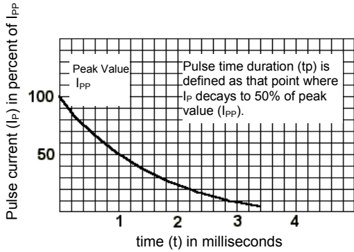
FIGURE 3 Pulse wave form for exponential surge
