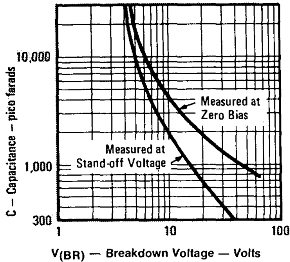
FIGURE 5 Typical Capacitance vs. Breakdown Voltage (Bidirectional Types)
