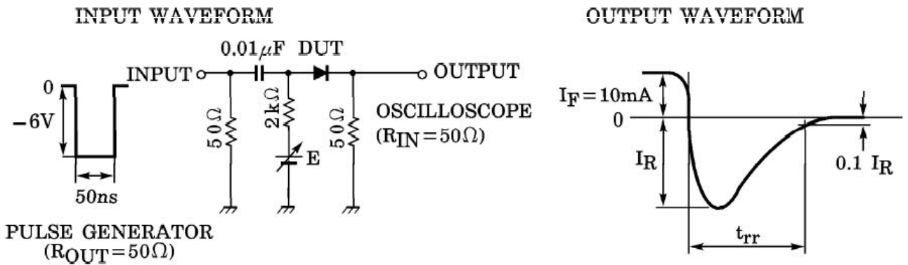
Fig.1 Reverse recovery time ( t_{rr} ) test circuit
