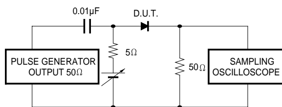
FIG. 6 - REVERSE RECOVERY TIME MEASUREMENT CIRCUIT
