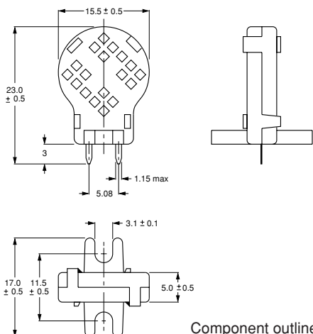
Component outline.
