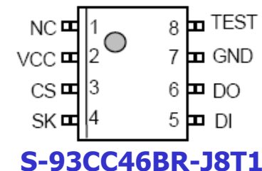
8-Pin SOP (JEDEC) (Rotated) Top view
