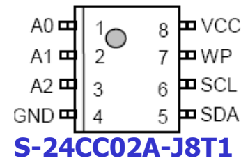
8-Pin SOP (JEDEC) Top view
