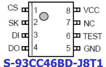
8-Pin SOP (JEDEC) Top view
