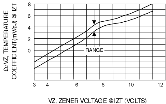
Fig. 5-UNITS TO 12 VOLTS
