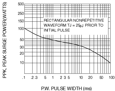
Fig. 3-MAXIMUM SURGE POWER
