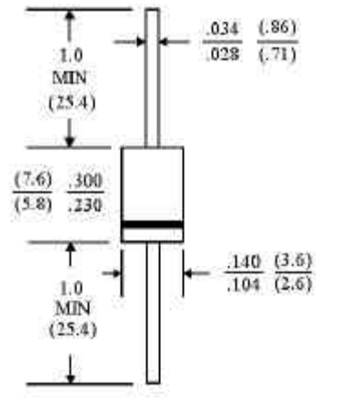
DO-15
