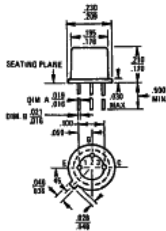
TO-18
