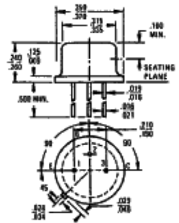
TO-39
