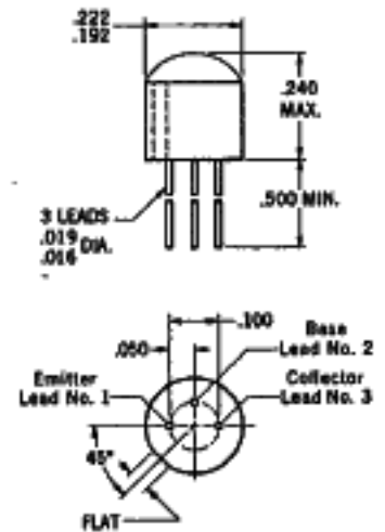
TO-106
