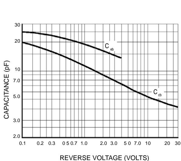
Figure 3. Capacitance
