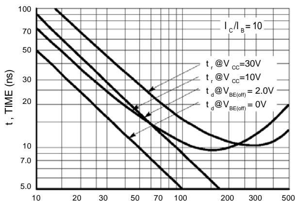
Figure 5. Turn-On Time
