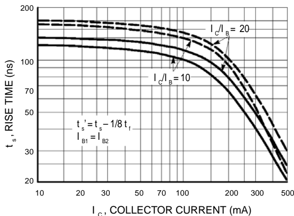
Figure 7. Storage Time
