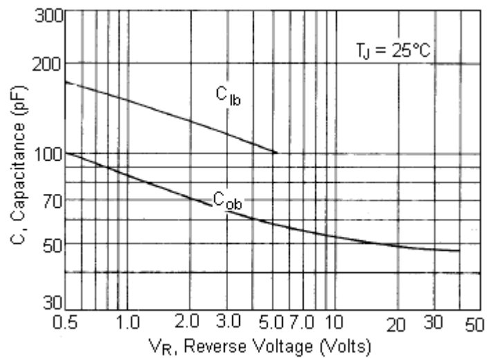
Figure 8 - Capacitances
