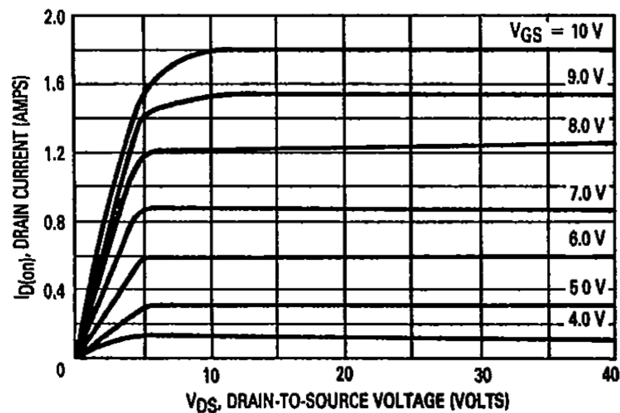
FIGURE 5 — OUTPUT CHARACTERISTICS
